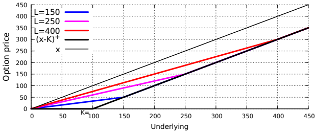
Fig. 15.5: American call prices by exercising at \tau_L for different values of L and K = 100 .
